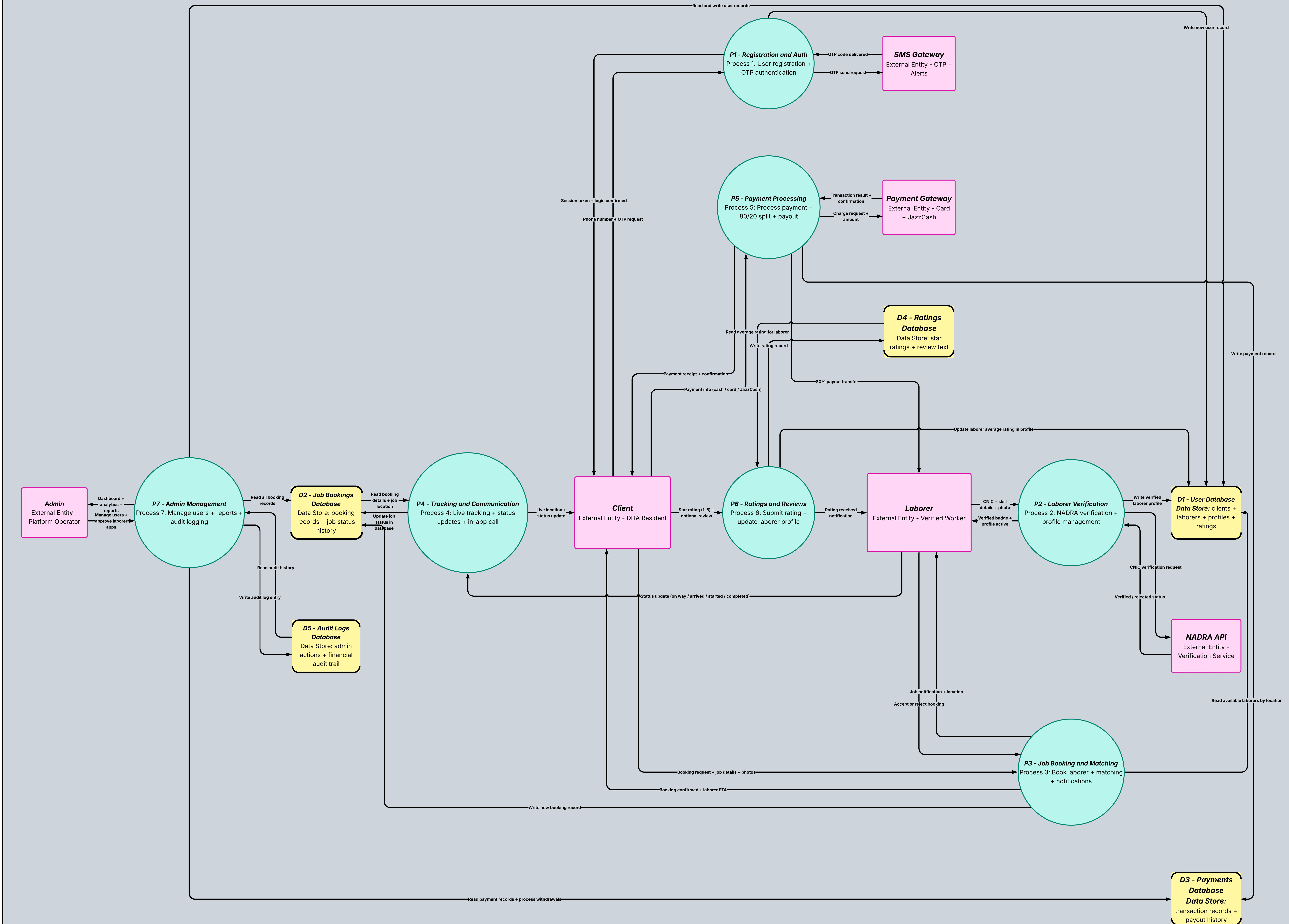
Figure 3. Karigar - DFD Level 1
